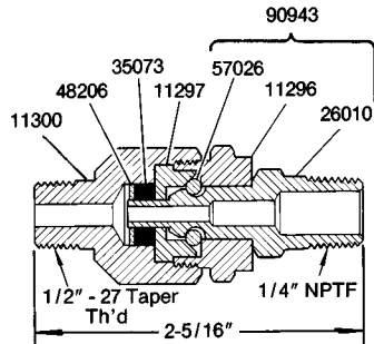
82399 STRAIGHT SWIVEL
