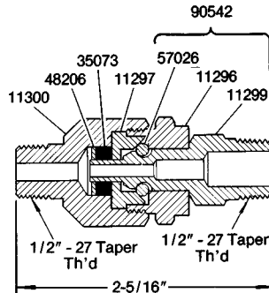
82080 STRAIGHT SWIVEL
