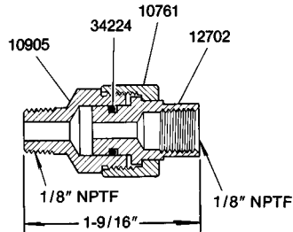
81606 STRAIGHT SWIVEL
