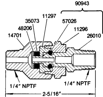
83938 STRAIGHT SWIVEL
