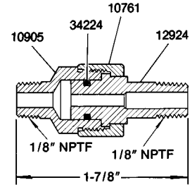
81703 STRAIGHT SWIVEL
