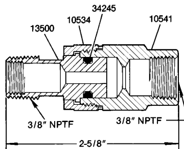
80353 STRAIGHT SWIVEL
